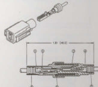
① 568-001-000-100 ② U TERMINAL ③ 568-001-000-100 ④ F TERMINAL ⑤ WIRE SEAL ⑥ HOUSING SEAL
